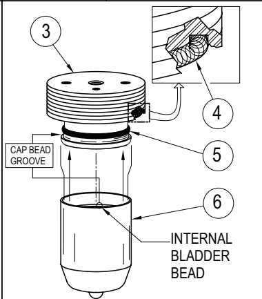
FIGURE 6 BLADDER & O-RINGS INSTALLATION
