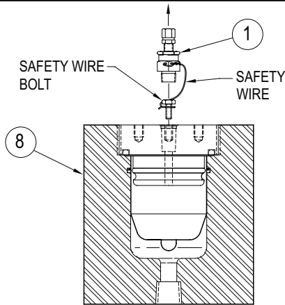
FIGURE 2 (CASE SHOWN IN SECTION VIEW)
